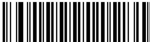
* Disable Code 11
